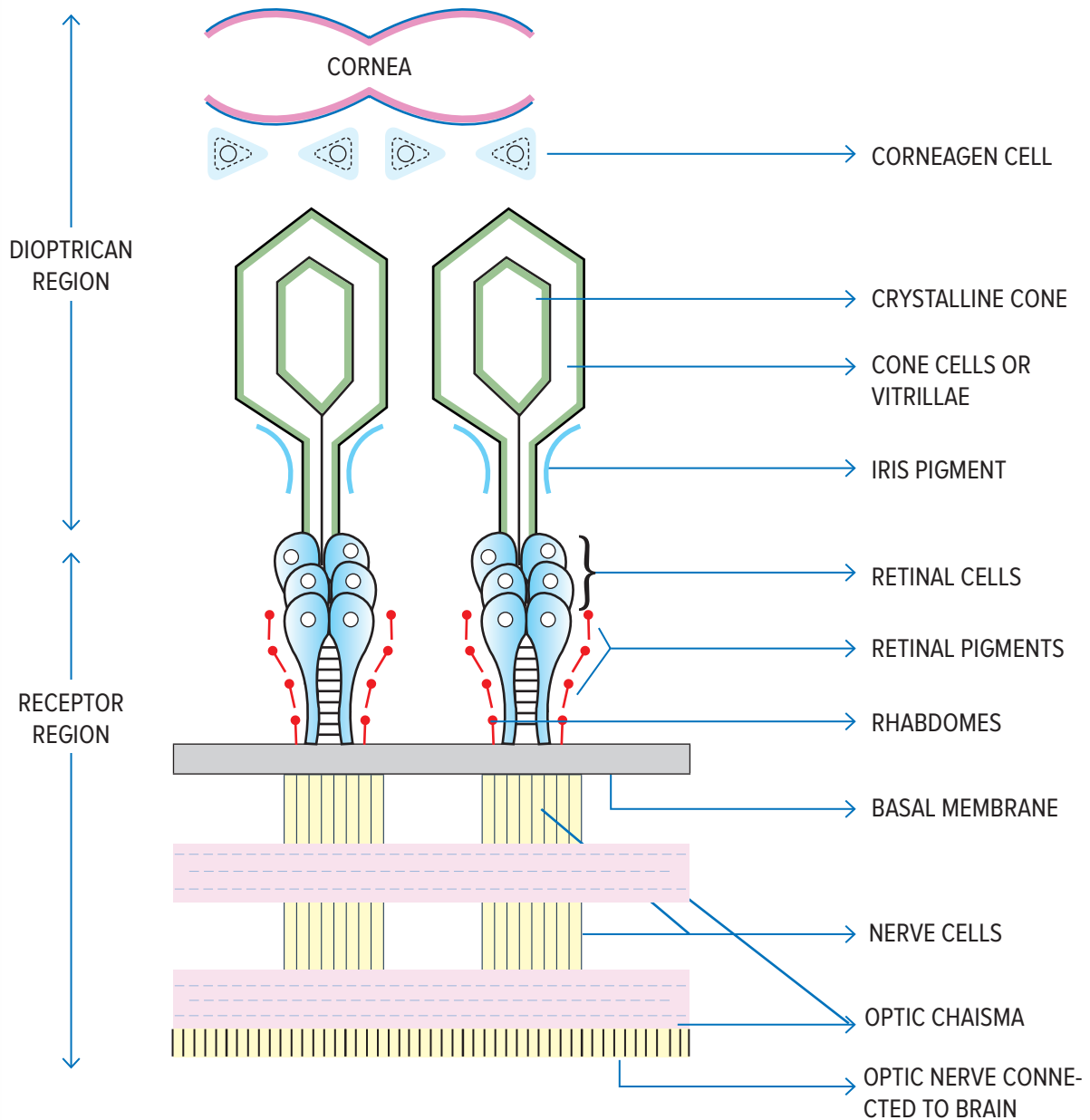
Fig: ▲ Structure of compound eye.
