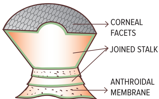
Fig: ▲ general appearance of a compound eye.
